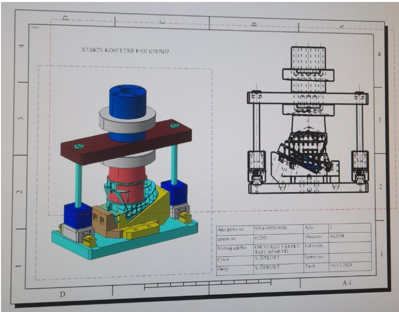
Test Apparate for Rubber Compound ( Fatigue )
